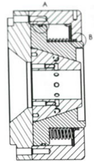
Section view
